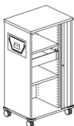
Height 1,090 mm, width 572 mm, depth 436 mm
